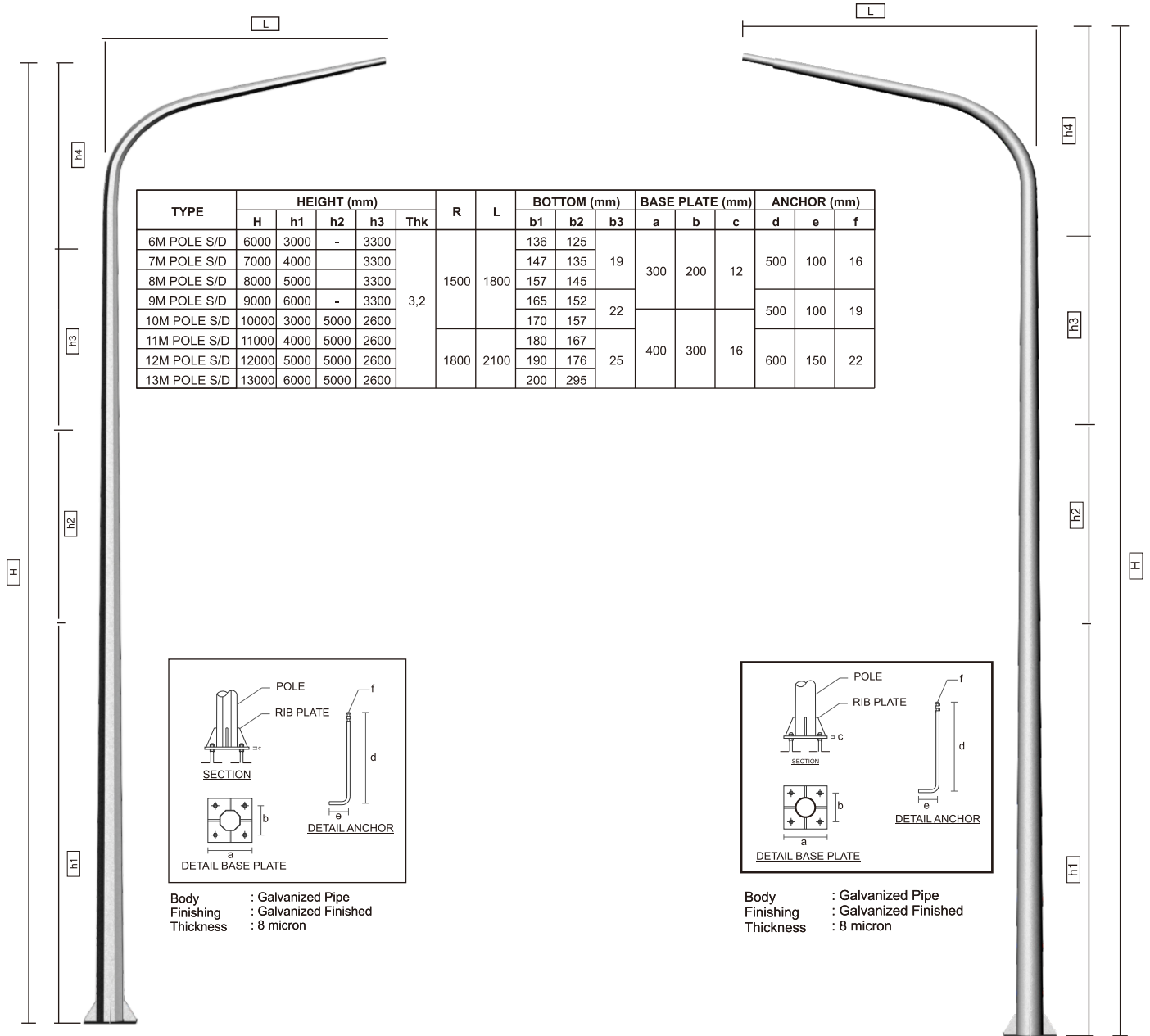
STANDART OCTAGON LIGHTING POLE
